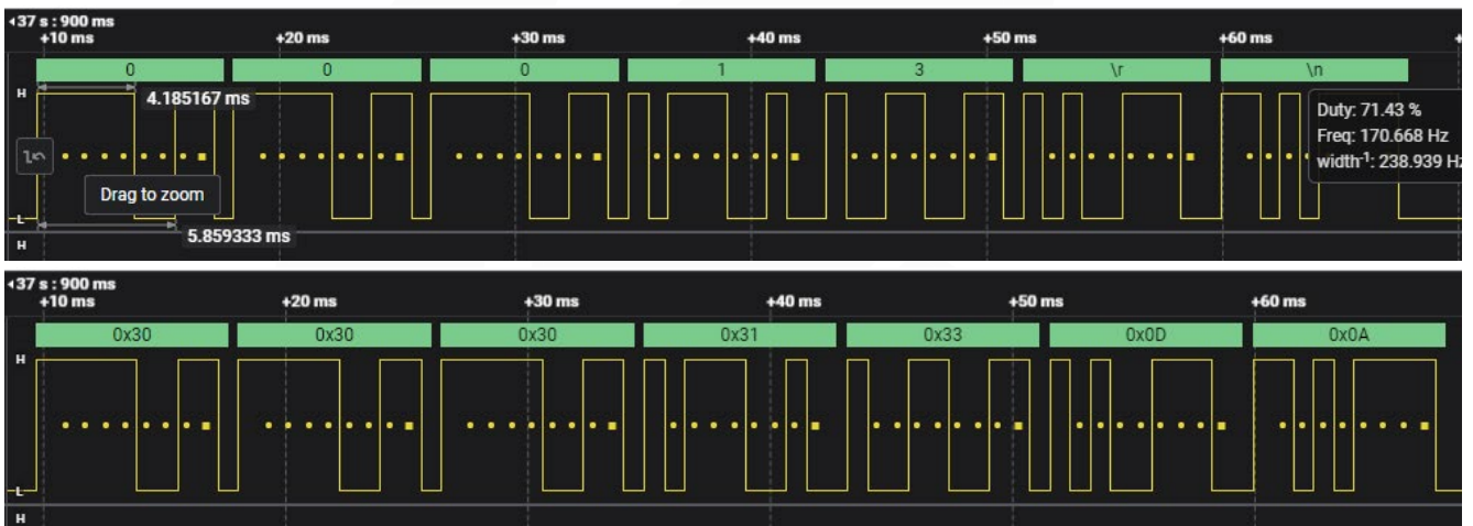
Figure 10. Oscillogram
